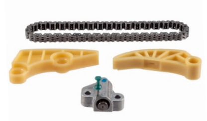
TS22772 INCLUDES OIL PUMP CHAIN SET COMPONENTS ONLY
